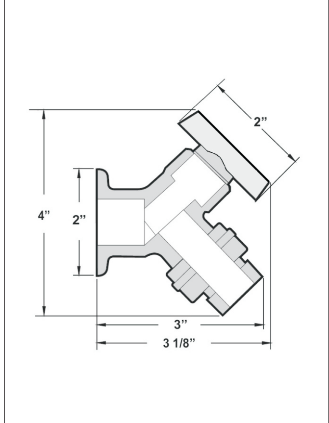
HY-9000 Series wall faucet dimensions
